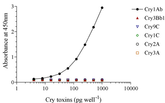
Fig. 2 – Cross-reactions of Cry toxins with Cry1Ab antibody using parallel standard concentrations in assay buffer in ELISA.
