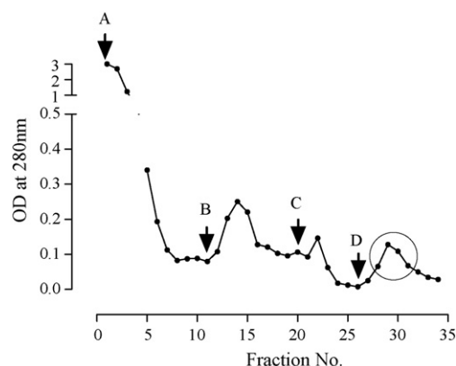
Fig. 1 – Immuno-affinity cleanup of antiserum collected from rabbit immunized against Cry1Ab protein. After applying antiserum onto affinity column, the column was washed with different wash buffers: A, PBS buffer pH 7.4; B, 0.5 \text{ mol L}^{-1} NaSCN buffer pH 8.0 and C, 0.1 \text{ mol L}^{-1} glycine buffer pH 3.5. Cry1Ab protein specific antibody (IgG) was eluted with buffer D ( 0.1 \text{ mol L}^{-1} glycine buffer pH 2.0). Eluted fractions 28–31 (marked in circle) containing specific antibody were pooled and further concentrated after dialysis.
