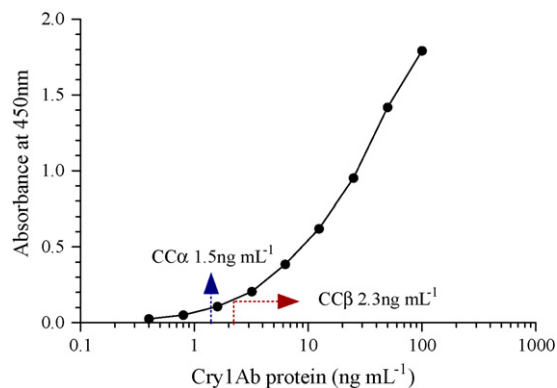
Fig. 3 – A typical matrix-matched calibration curve for Cry1Ab protein in bovine blood plasma.
