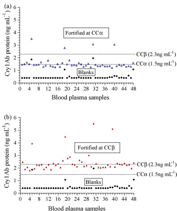
Fig. 4 – (a) Determination of detection capability (CC \beta ) of the Cry1Ab protein ELISA in bovine blood plasma. Detection capability was calculated from the Cry1Ab protein fortified blanks ( \Delta ; n = 48 ) at the concentration level of decision limit (CC \alpha 1.5 ng mL -1 ). CC \alpha calculated as three times S/N ratio from the blanks ( \bullet : blood plasma collected from 48 cows fed non-transgenic ration). (b) Determination of \alpha - and \beta -errors for the Cry1Ab protein ELISA in bovine blood plasma. \alpha -Error and \beta -error was calculated from the Cry1Ab toxin fortified blanks. Percentage of blanks ( \bullet : blood plasma from 48 cows fed non-transgenic ration) lying above the decision limit (CC \alpha 1.5 ng mL -1 ) indicated the \alpha -error (>5%). \beta -error (zero) was indicated by the spiked blanks ( \Delta ; n = 48 ) at concentration level of 2.3 ng mL -1 (CC \beta ).
