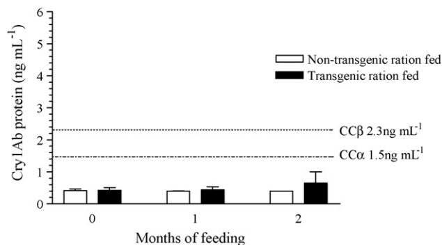
Fig. 5 – Cry1Ab toxin ELISA background signals in blood plasma of cows fed transgenic ( n = 8 ) and non-transgenic ration ( n = 7 ). Blood samples collected before and, after 1 and 2 months of feeding were investigated for the presence of the Cry1Ab protein. No sample found positive for the presence of Cry1Ab toxin in plasma and all the values were below the decision limit ( 1.5 \text{ ng mL}^{-1} ) and detection capability ( 2.3 \text{ ng mL}^{-1} ). The data is presented as mean ( \pm S.D.) values.
